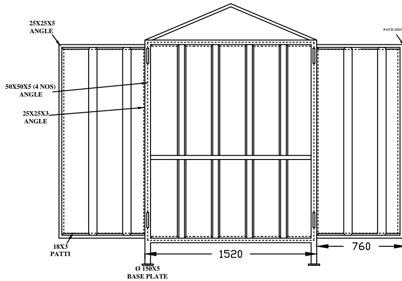
FRONT OPEN VIEW
