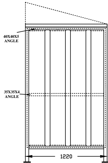
LEFT HAND SIDE VIEW
